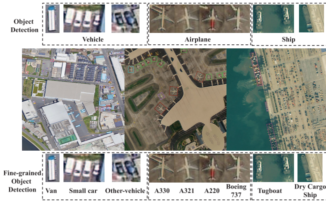
Fig. 1. Comparison between ordinary remote sensing target detection and fine-grained remote sensing target detection.
