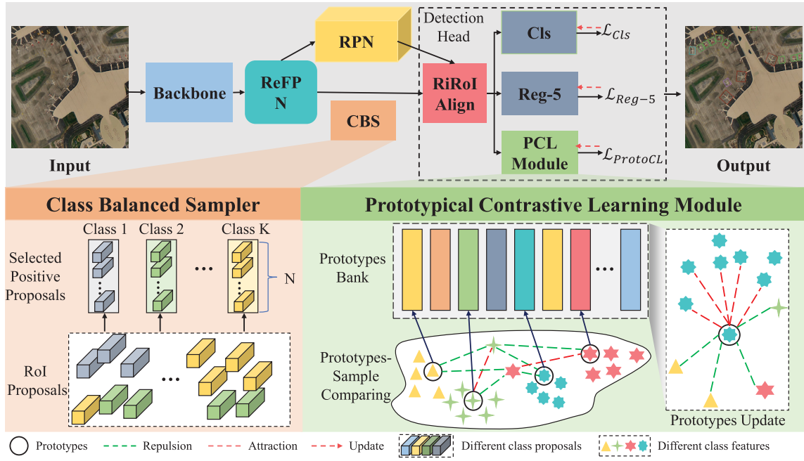
Fig. 2. Framework of the proposed PCLDet. For input remote sensing images, the PCLDet first applies the ReResNet50 backbone and ReFPN in order to extract features. Then, the PCLDet utilizes the CBS in RPN to generate proposals. After that, the PCL module increases fine-grained target interclass distances by contrasting prototype and sample features. Finally, the PCLDet updates the prototypes in the prototypes bank with the ProtoCL loss.
