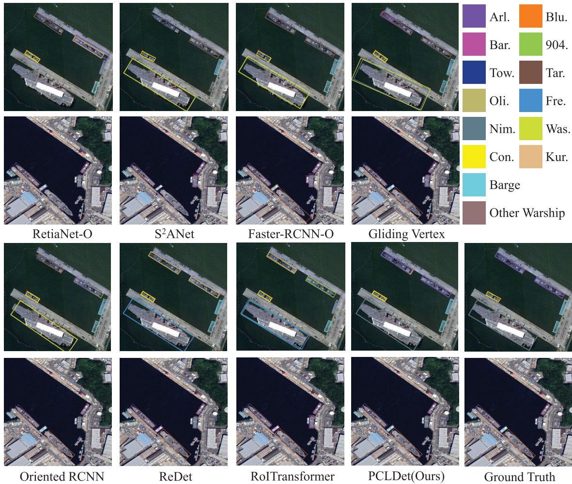
Fig. 5. Visualization of compared SOTA methods results on OFSD. The category abbreviations are given as follows: Arleigh Burke-class Destroyer (Arl.), Blue Ridge class command ship (Blu.), Barracks Ship (Bar.), Towing vessel (Tow.), Oliver Hazard Perry-class frigate (Oli.), Nimitz Aircraft Carrier (Nim.), Container Ship (Con.), Tarawa-class amphibious assault ship (Tar.), Freedom-class littoral combat ship (Fre.), Wasp-class amphibious assault ship (Was.), Kurobe-class training support ship (Kur.), and 904-general stores issue ship (904.)
