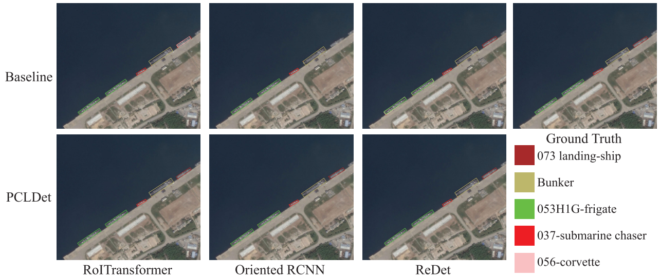
Fig. 6. Visualization of detection results on OFSD, using baseline (the first row) and the PCLDet (the second row).
