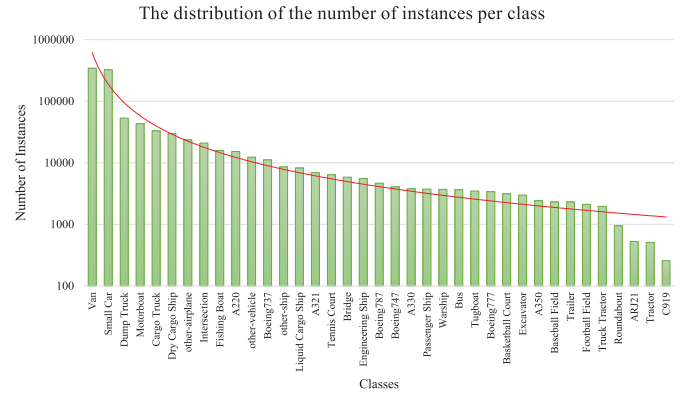
Fig. 3. Distribution of remote sensing fine-grained detection dataset Fari1M instances.
